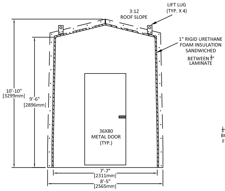
FRONT ELEV.
