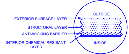
LAMINATE DETAIL
