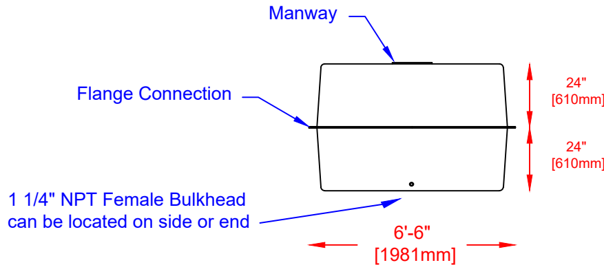
END VIEW
