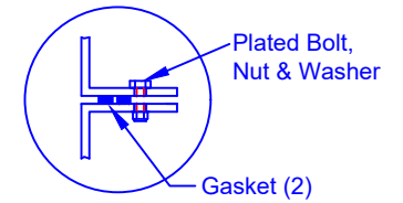
FLANGE CONNECTION DETAIL
