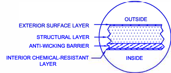
LAMINATE DETAIL
