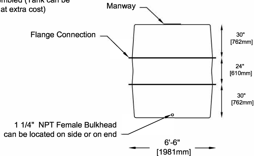
END VIEW
