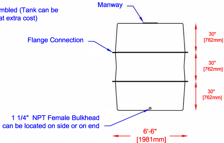
END VIEW
